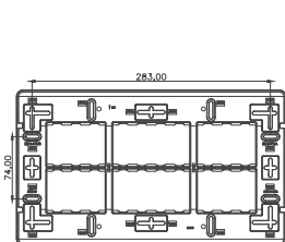
Cutout size— 253mm x 112mm Code No: 373015 20 module — 7.5" X 13"
