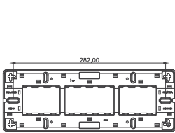
Cutout size— 251mm x 57mm Code No: 373009 10H module — 4.5" X 13"
