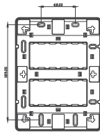
Cutout size— 130mm x 116mm Code No: 373019 10SQ module — 7" X 9"
