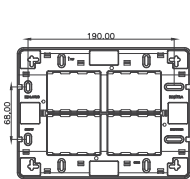
Cutout size— 151mm x 112mm Code No: 373012 12SQ module — 7" X 9"
