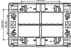
Cutout size— 196mm x 112mm Code No: 373013 16 module — 7.5" X 11"
